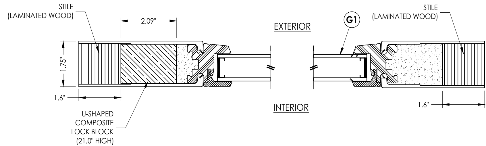
1 3 HORIZONTAL CROSS SECTION
